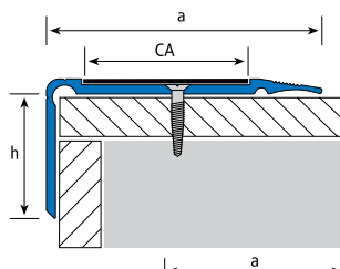
CA (Cinta antideslizante / Anti-slip tape)
